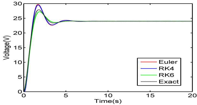
Figure 4: Comparison of Euler, RK4, RK6 and Exact solution for parallel circuit.
